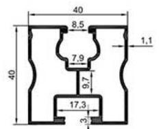
C1585 0.743 kg/m
