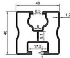
C1564 0.813 kg/m
